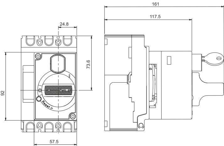
Dimensions with Rotary Handle-Direct
