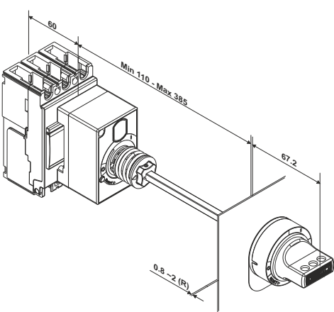
Dimensions with Rotary Handle-Vari-Depth
