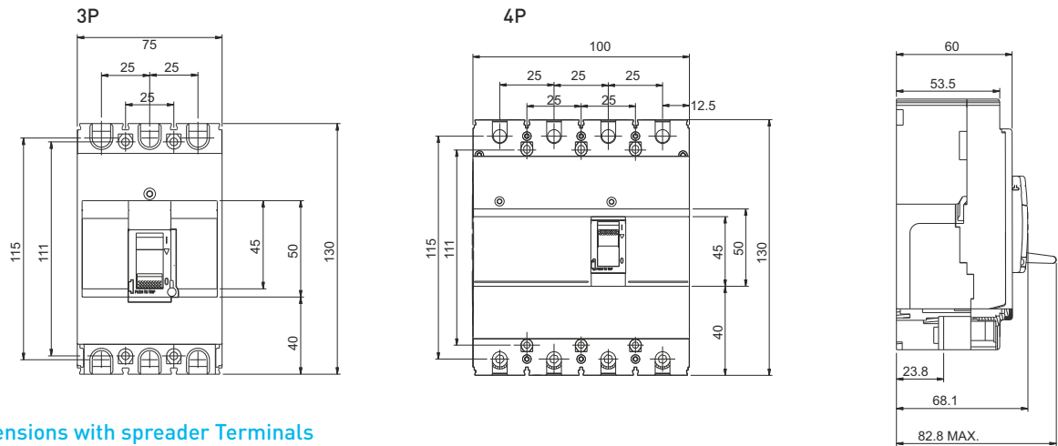
Overall and Mounting Dimensions
